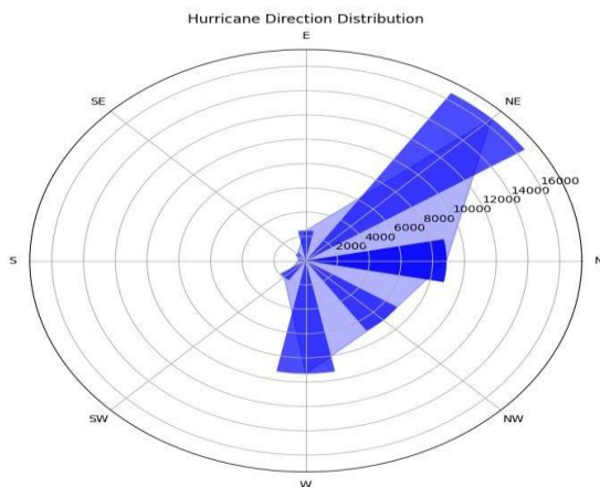
Figure 25: Polar Plot of Hurricane Directions.
