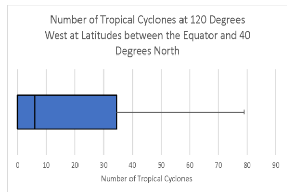
Figure 8: Box Plot [11].
