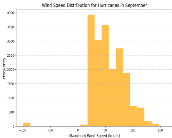
Figure 16: Bar Chart of Wind Speed Distribution for Hurricanes in September.
