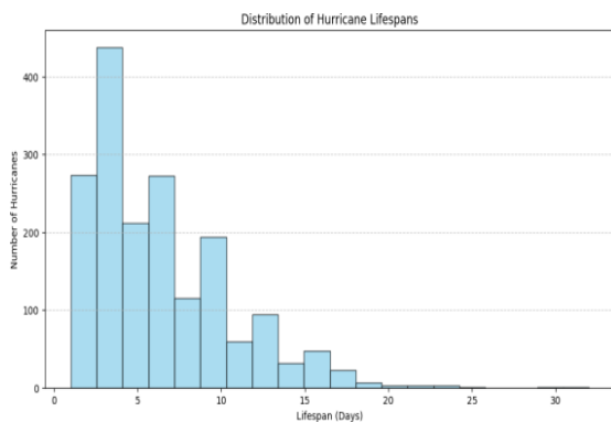
Figure 23: Histogram of Hurricane Lifespans.
