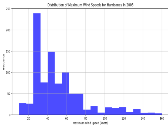
Figure 12: Bar chart of analyzing the distribution of wind speed for 2005.
