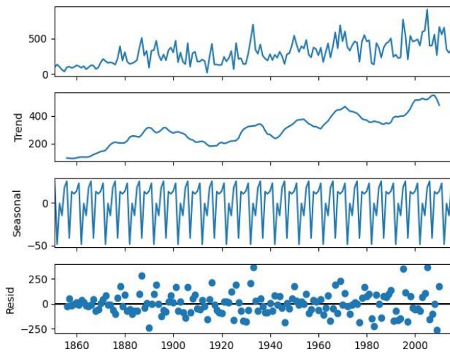
Figure 29: Time Series Decomposition of Hurricane Counts Over Years.
