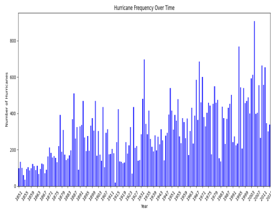
Figure 10: Bar Chart of Hurricane Frequency by Year.
