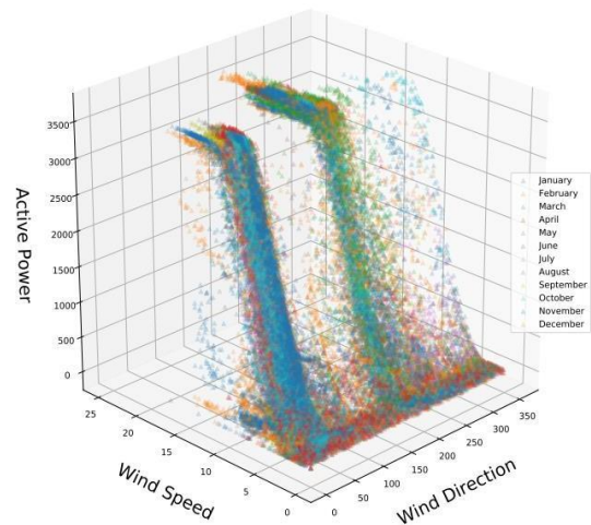
Figure 7: Scatter Plot
