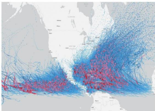
Figure 6: Geospatial Visualization [13].
