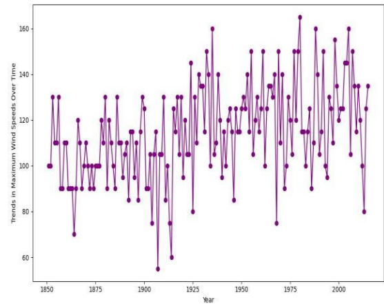
Figure 11: Line Plot of Maximum Wind Speeds Over Time.
