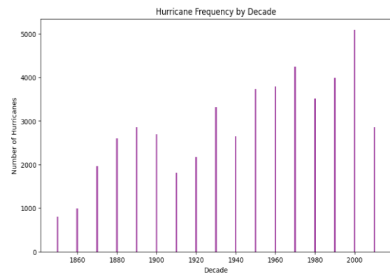
Figure 13: Bar Chart of Hurricane Frequency by Decade.
