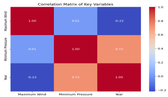
Figure 21: Correlation Matrix.
