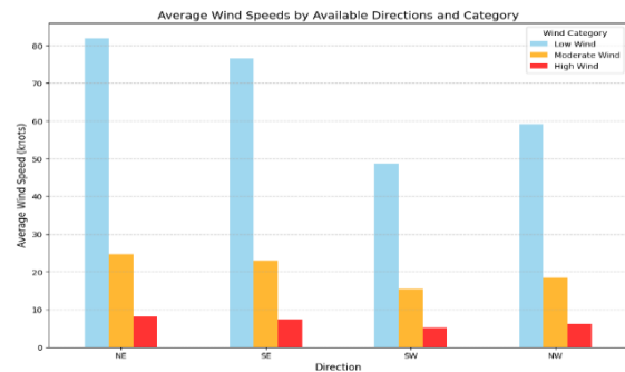
Figure 26: Bar Chart of Average Wind Speeds by Directions.
