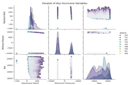
Figure 22: Pairplot.
