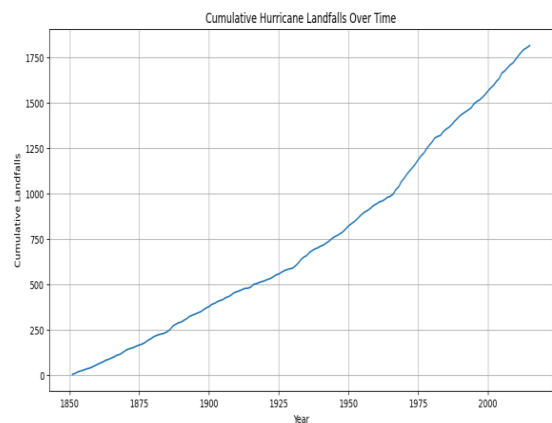
Figure 24: Line Plot of Cumulative Hurricane Landfalls.
