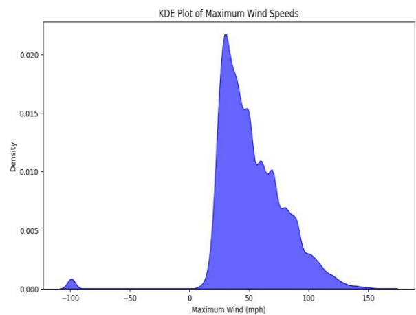
Figure 28: Kernel Density Estimation (KDE) Plot.
