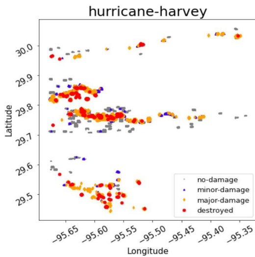
Figure 9: Cluster Analysis [12].
