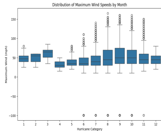
Figure 17: Box Plot of Maximum Wind Speeds by Month.
